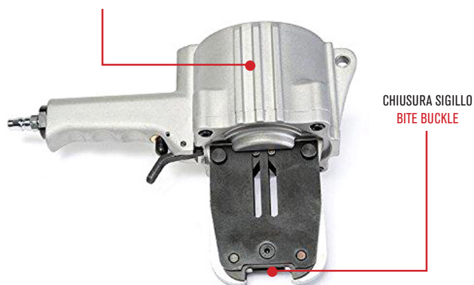
CILINDRO ARIA AIR CYLINDER
